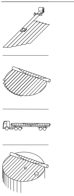
Complete prefabrication of the membrane in the plant
